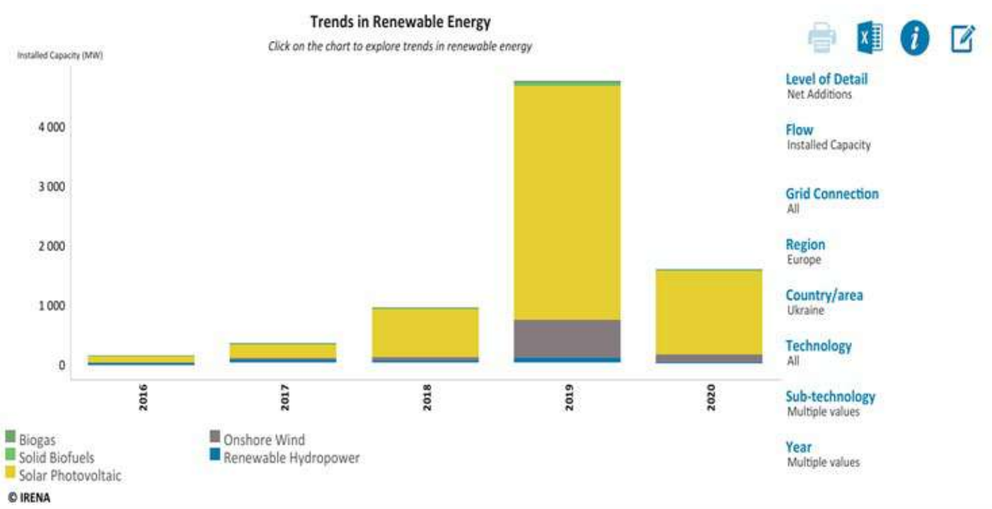
Fig. 18. Information of installed capacity in Ukraine for different renewable technologies in 2016-2020 (Source: author’s research results with using database IRENA)
